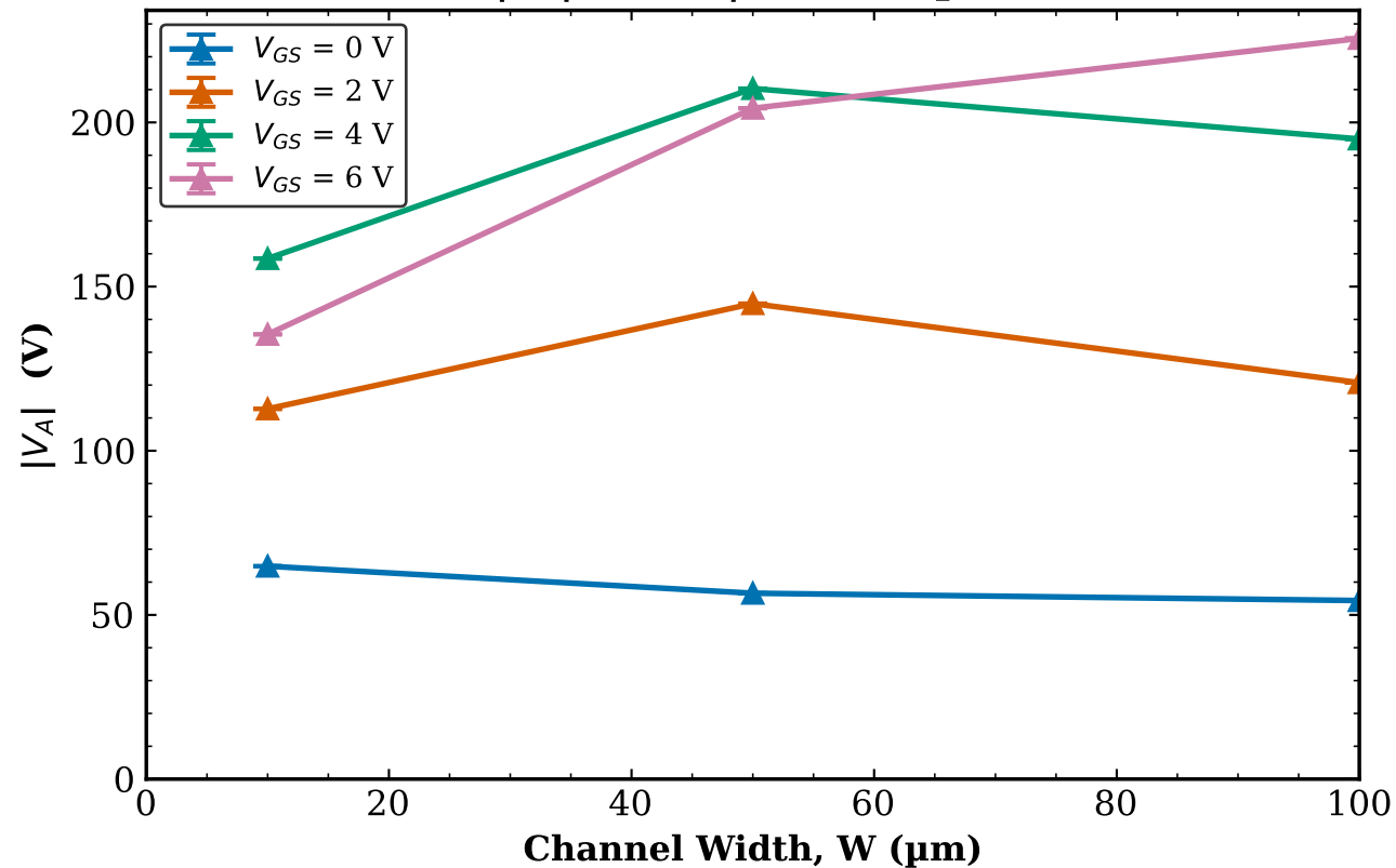
TFT1 Transistor 2 |V_A| vs W | L = 40\text{ }\mu\text{m}
